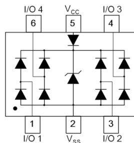
Device Schematic
